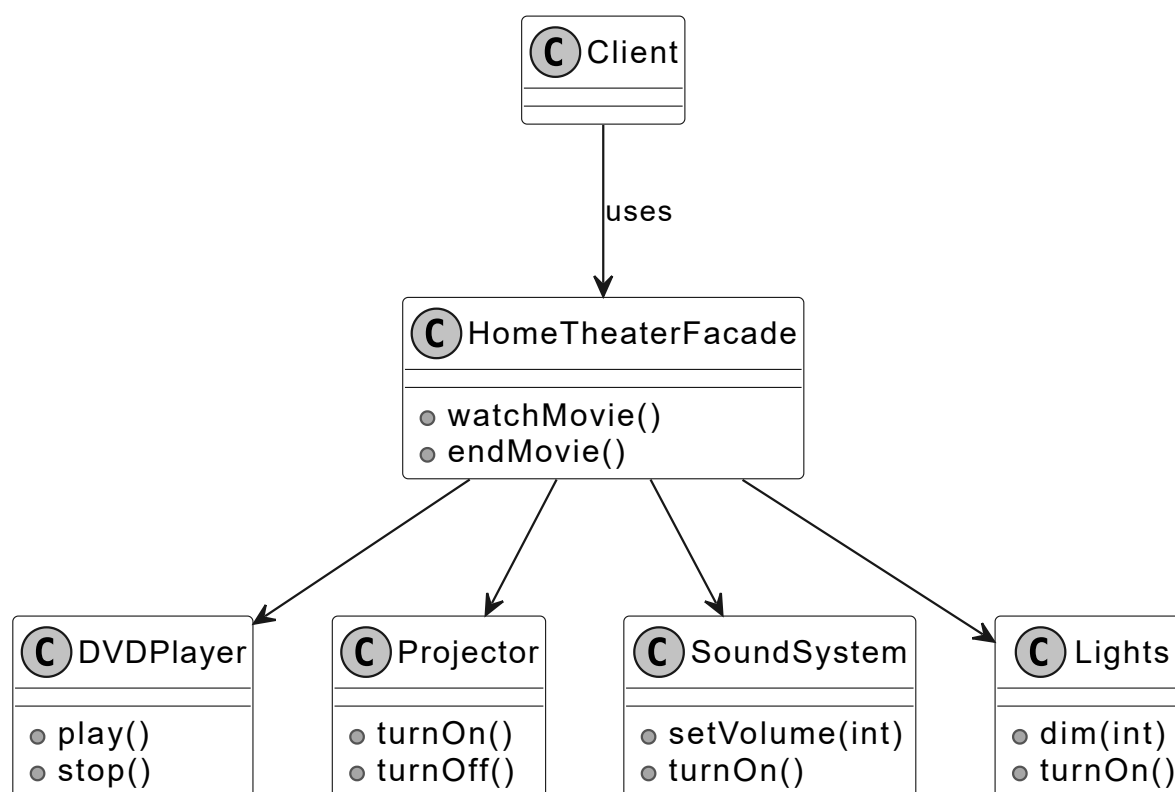
Facade design pattern class diagram
