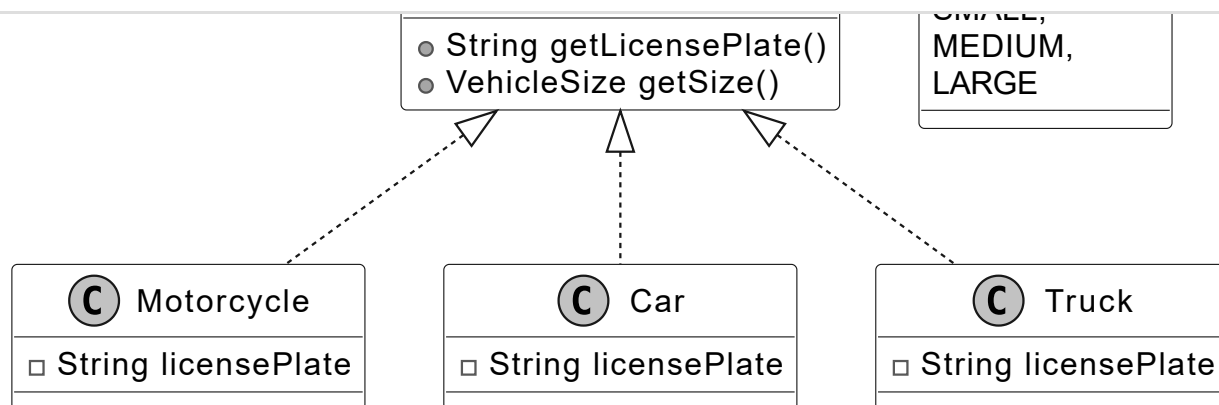
Vehicle and its concrete classes
