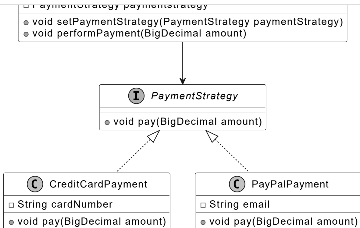
Strategy design pattern class diagram
