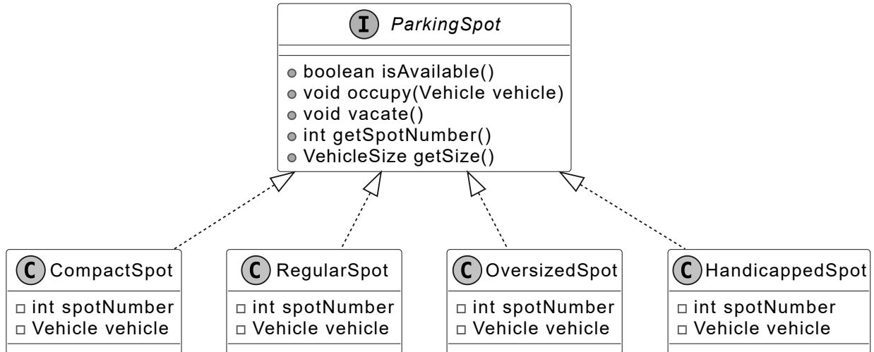
ParkingSpot with HandicappedSpot class
