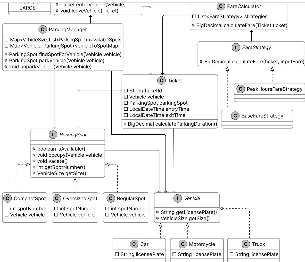
Class Diagram of Parking Lot
