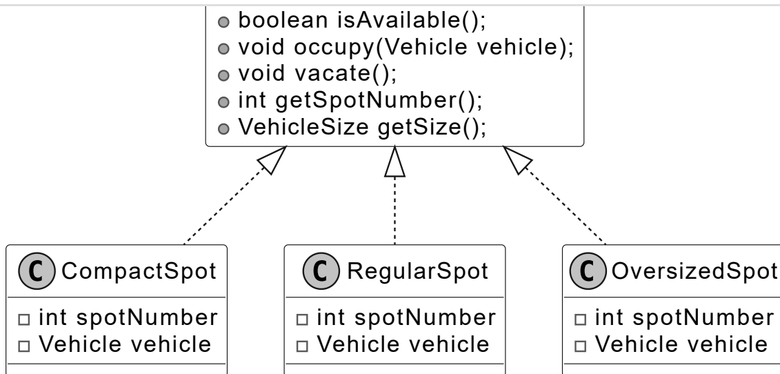
Parking Spot and its concrete classes
